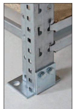
Frames are fixed down through bolt on footplates.
