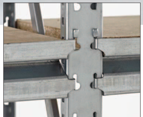
22mm chipboard shelves fit flush to the top of the beam making loading snag free.
