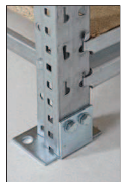
Frames are fixed down through bolt on footplates.
